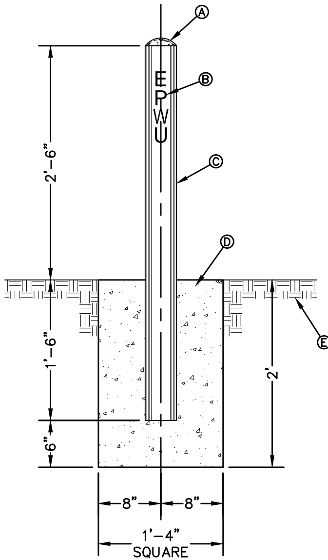
MARKER POST
