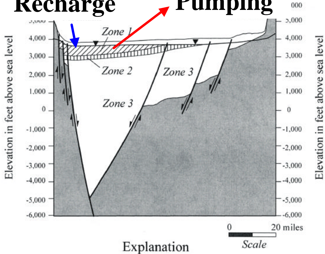
Figure 6-16 Subregional Groundwater Budget Components (Cross-Section View)
