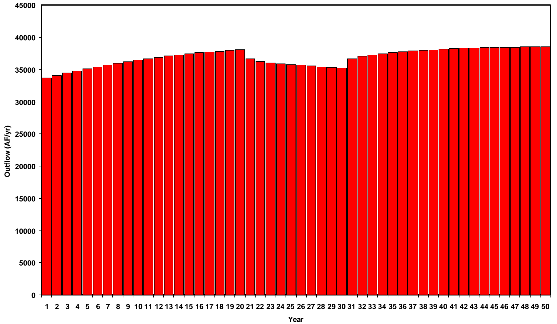
Figure 7-33 El Paso Area - Outflow to Juarez JDF Scenario
