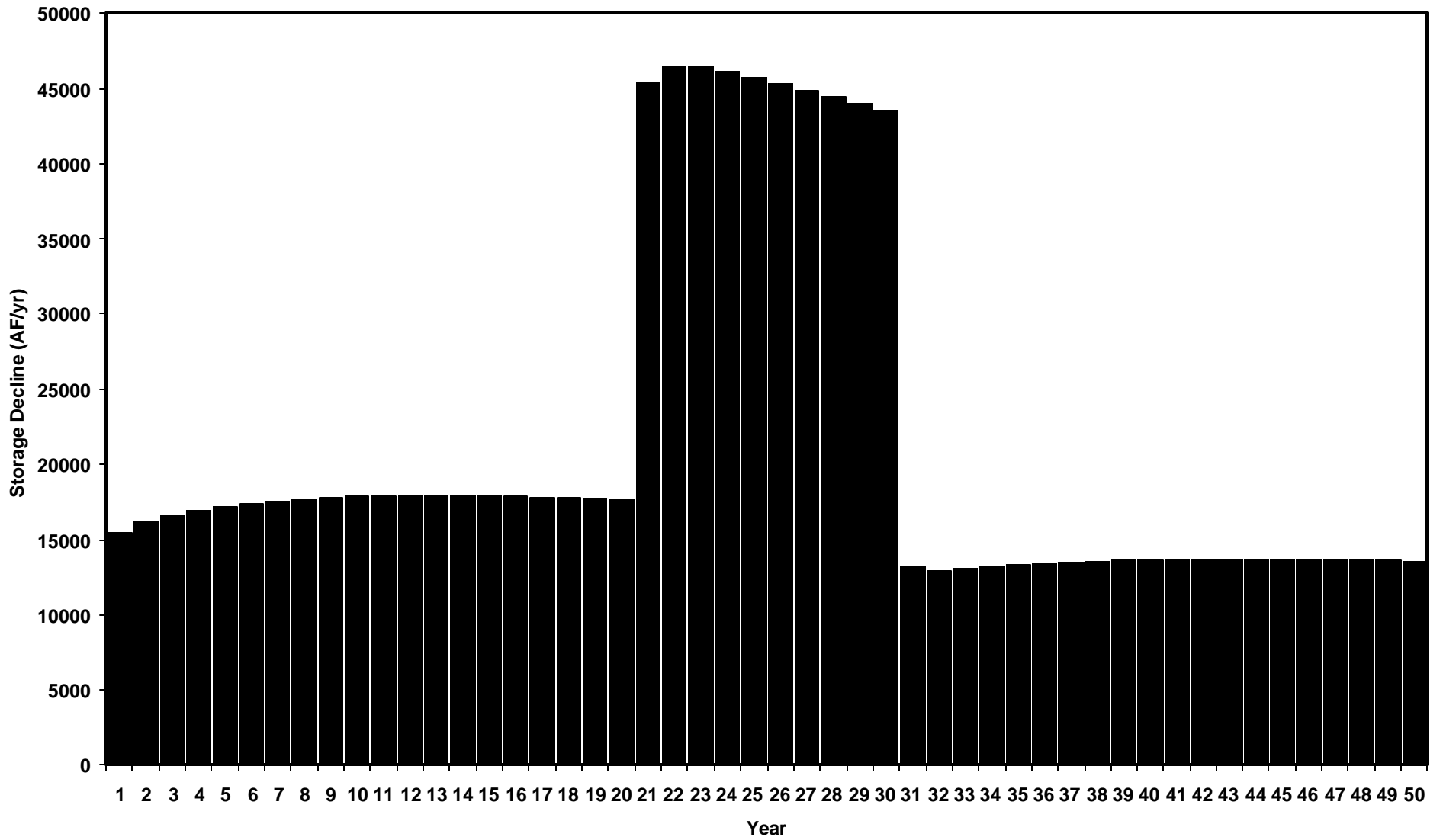
Figure 7-34 El Paso Area Storage Decline JDF Scenario
