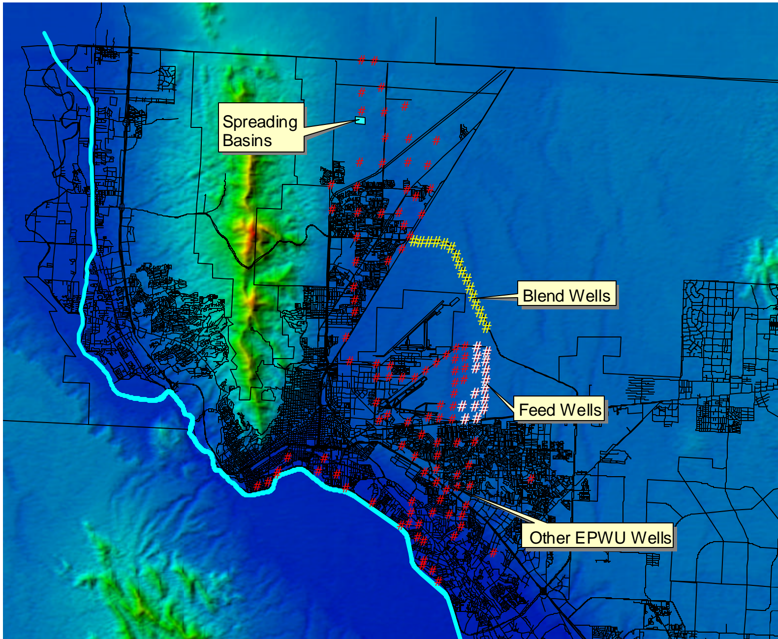
Figure 7-35 Location of Spreading Basins and JDF Wells
