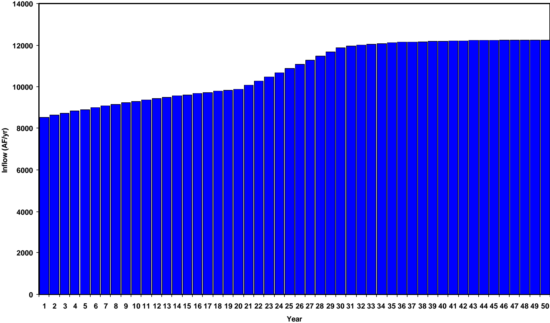
Figure 7-31 El Paso Area - Inflow from East JDF Scenario
