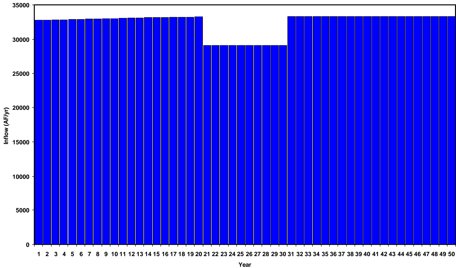
Figure 7-32 El Paso Area - Inflow from Surface Water JDF Scenario
